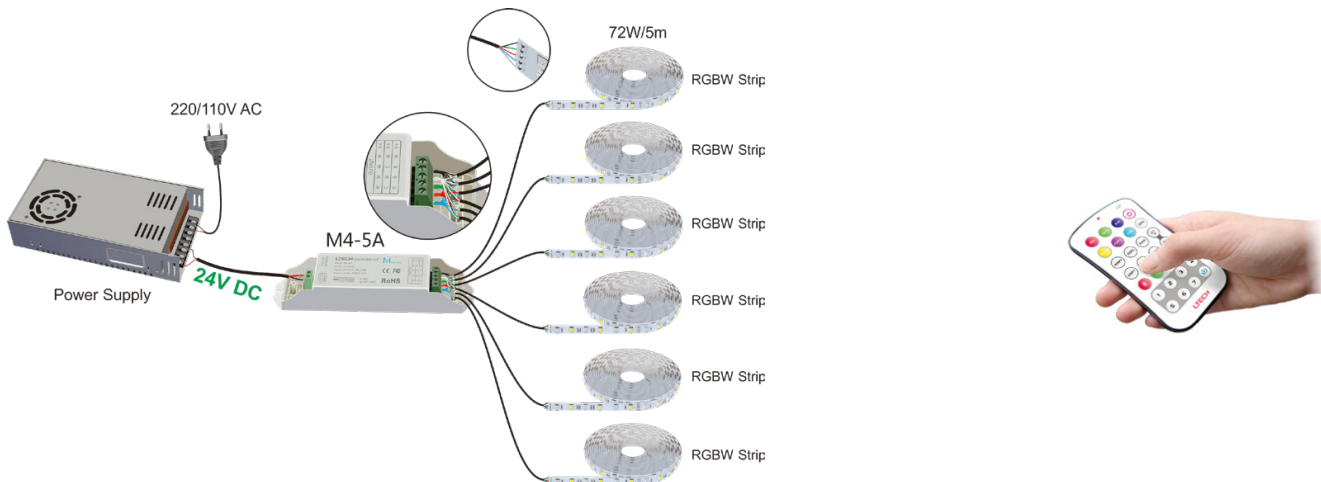
E.g. 2: Connected 24V lamp, loads 1~480W (5A×4CH×24V).
